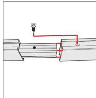
Spline Connection
